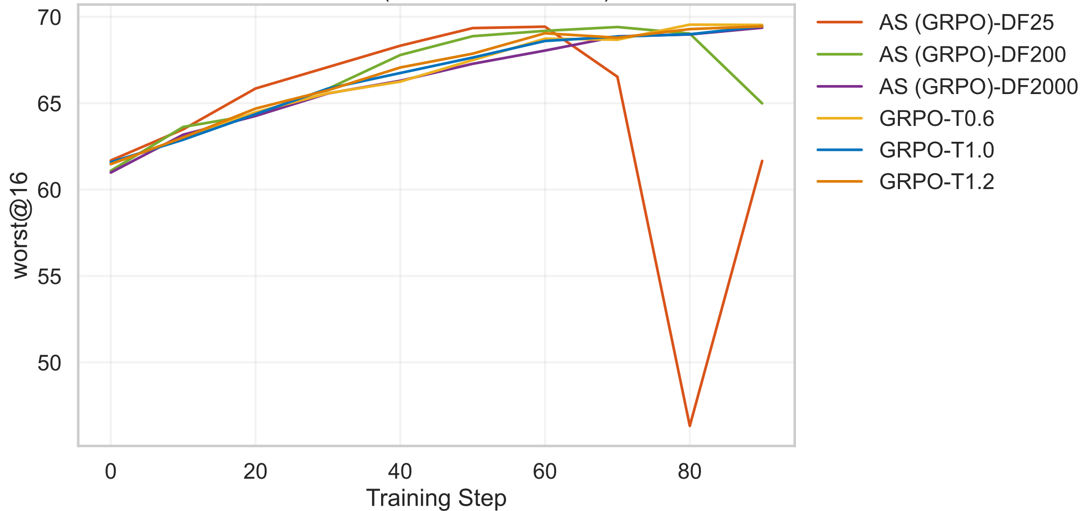
MATH-500 (Qwen2.5-Math-1.5B)
