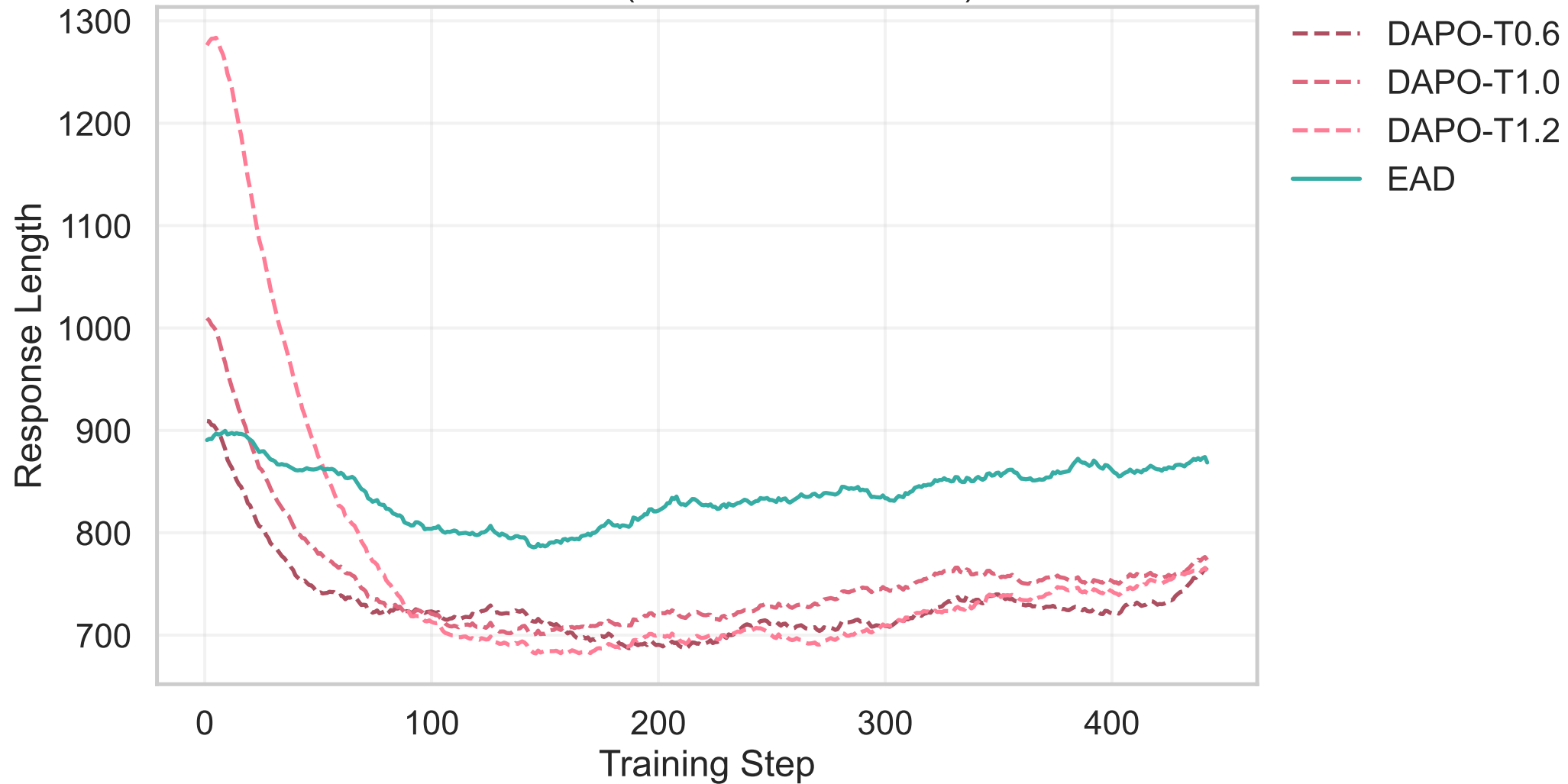
MATH-500 (Qwen2.5-Math-1.5B)
