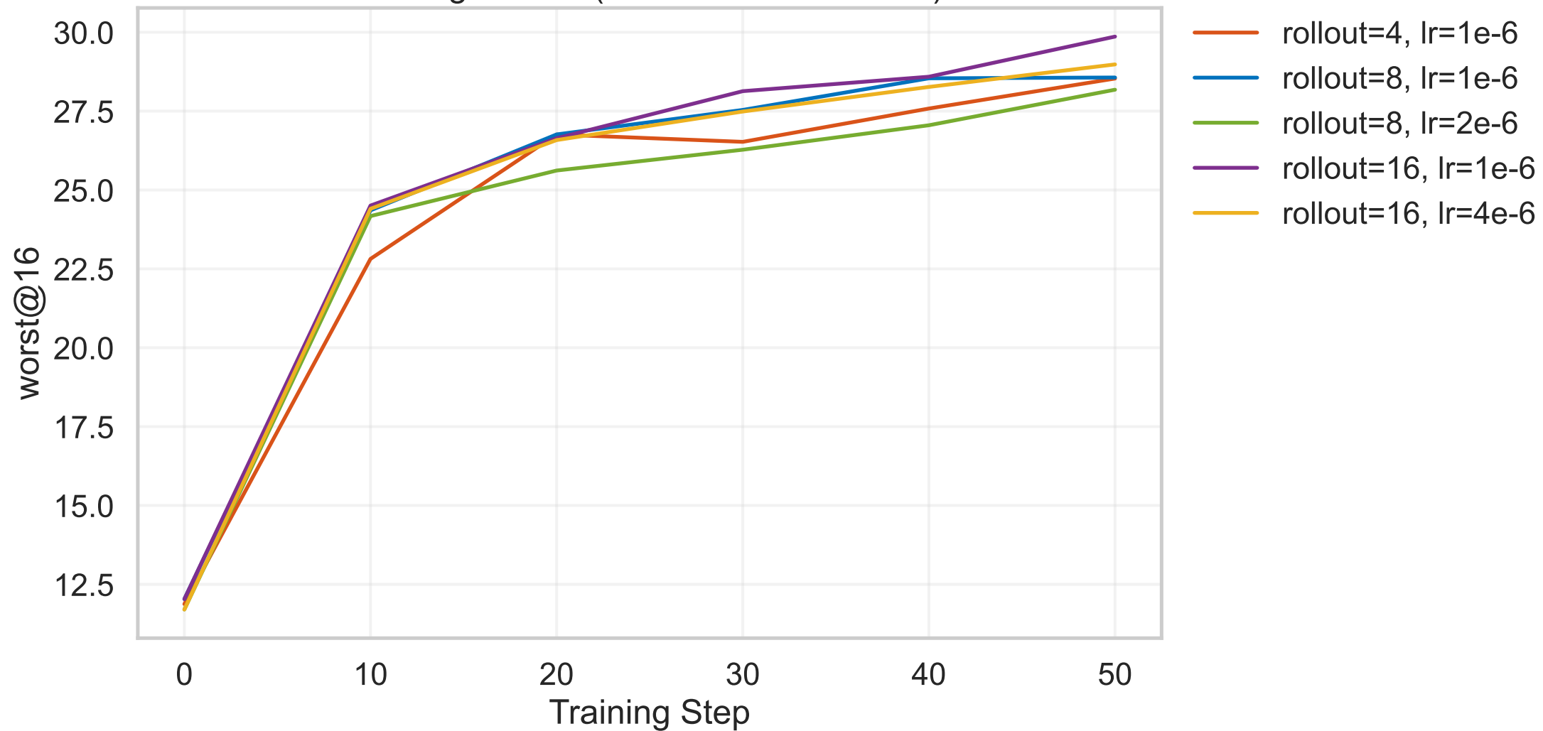
Scaling Rollout (Llama-3.2-1B-Instruct)
