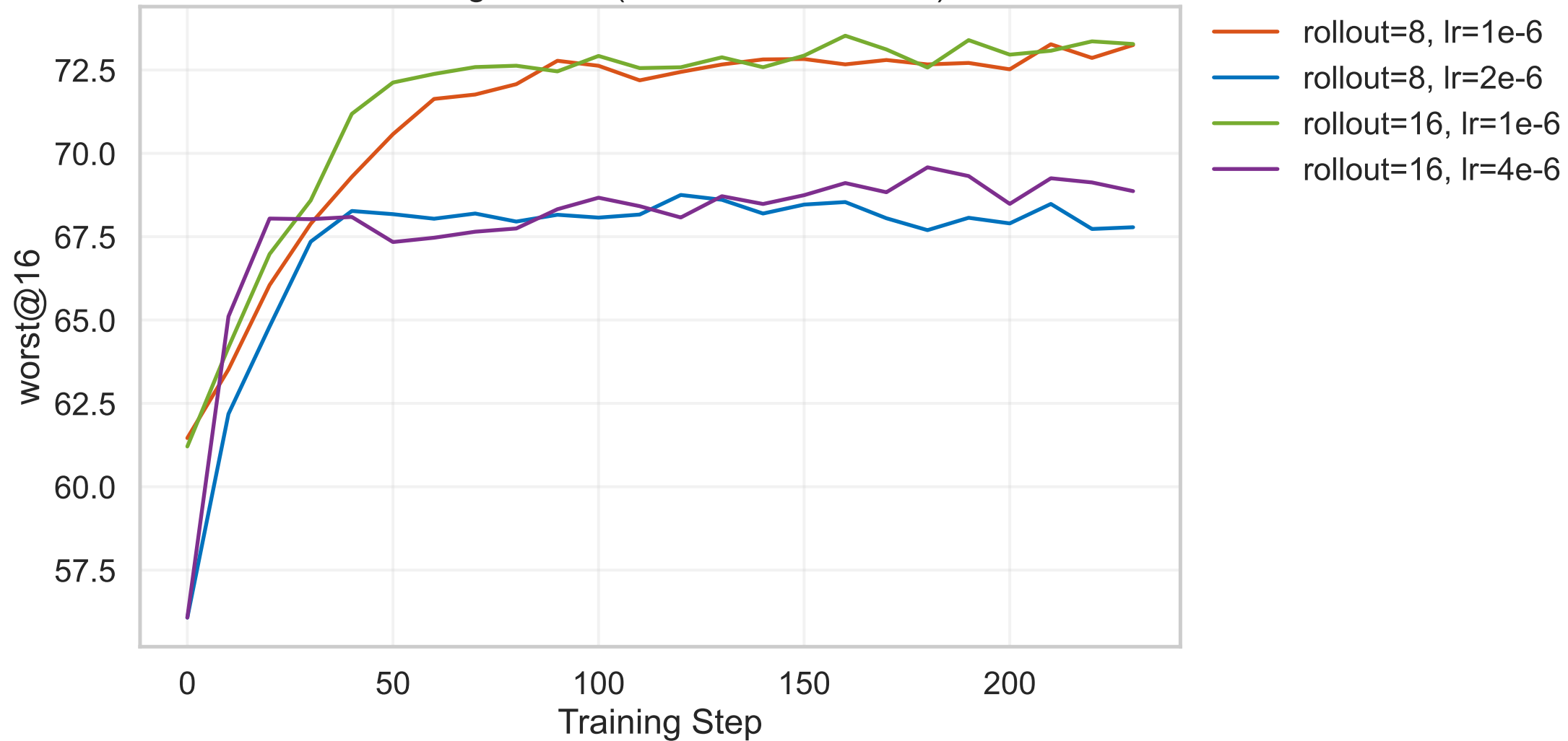
Scaling Rollout (Qwen2.5-Math-1.5B)
