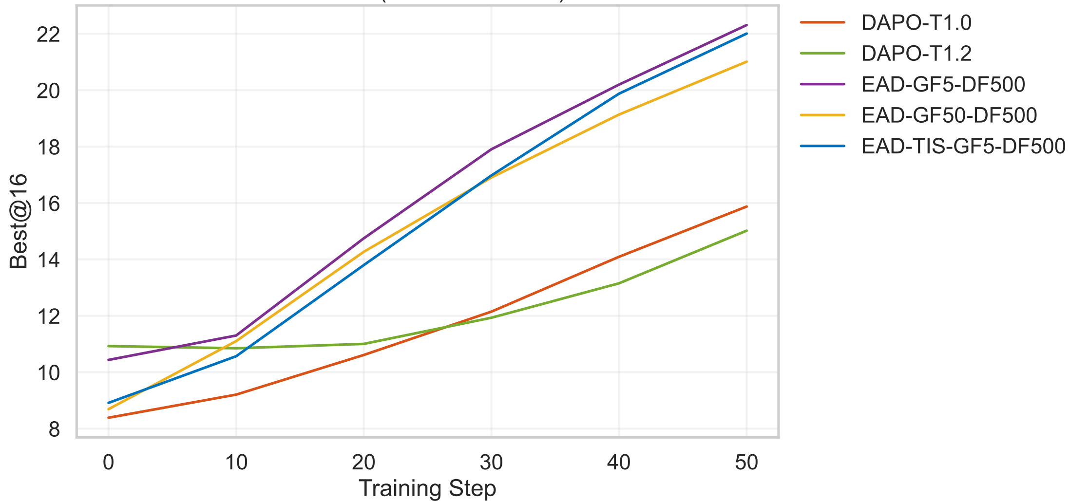
AIME24 (Qwen3-8B-Base)
