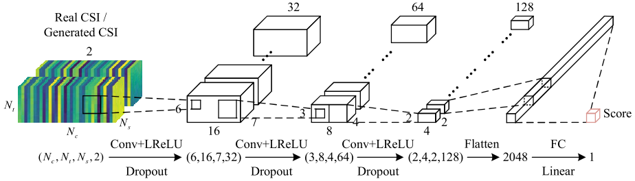
(b) Discriminator
