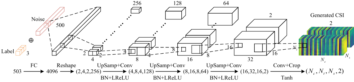
(c) Generator
