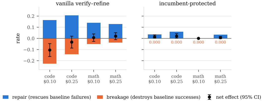
Figure 1: The same experiment, read two ways. Left: a standard verify-refine workflow repairs many tasks the baseline fails (blue, above the axis) and destroys many the baseline solves (orange, below), so the net effect (black, 95% CI)—the quantity the literature reports—is small and can take either sign. Right: protecting the incumbent answer removes the lower term entirely and the same machinery becomes a small, reliable gain. Frozen test splits, three execution seeds, matched hard budgets; panels share an axis.
