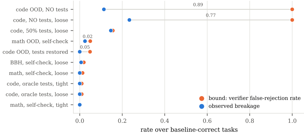
Figure 3: The bound equation 5 against measurement, in every condition we ran. Its left-hand side is a property of the verifier alone and can be measured without executing the workflow: a gated workflow that exits after its verifier accepted the draft leaves a different trace from one that proceeds to refine, so the false-rejection rate is recoverable from logs already collected. Observed breakage falls below the bound in all ten conditions — as it must, if the premise holds — across the full range from a verifier that almost never rejects a correct draft (0.009) to one that rejects every draft because it has no information (1.000). The figure is a check on the implementation and a reading of the bound’s slack, not a test of a contingent law. The bound is nearly tight where the verifier is moderately noisy—breakage 0.146 against a bound of 0.156 under 50% test masking—and loose where it is uninformative, because refinement sometimes recovers an answer it has just discarded. Rates are over baseline-correct tasks.
