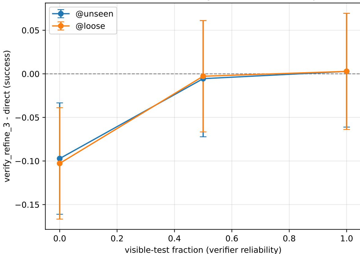
code: structure advantage vs verifier reliability
