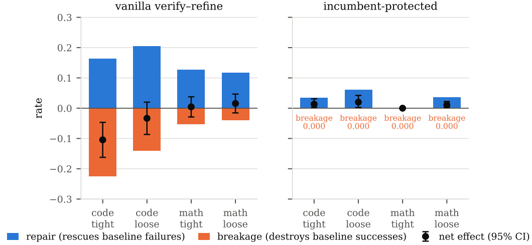
Figure 1: The same experiment, read two ways. Left: a standard verify-refine workflow repairs many tasks the baseline fails (blue, above the axis) and destroys many the baseline solves (orange, below), so the net effect (black, 95% CI)—the quantity the literature reports—is small and can take either sign. Right: protecting the incumbent answer removes the lower term entirely and the same machinery becomes a small, reliable gain. Frozen test splits, three execution seeds, matched hard budgets; panels share an axis.
