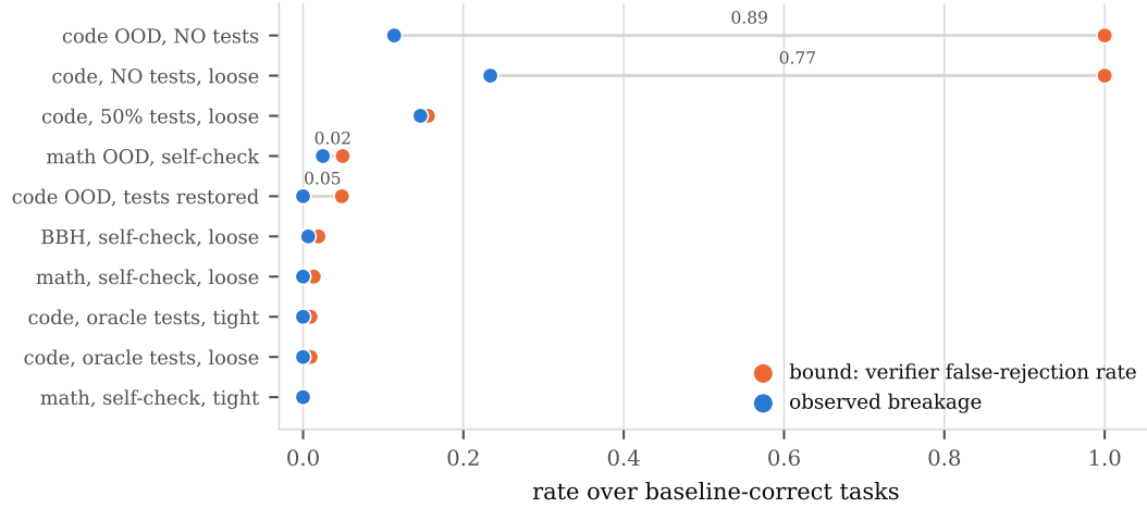
Figure 3: The bound equation 4 against measurement, in every condition we ran. Its left-hand side is a property of the verifier alone and can be measured without executing the workflow: a gated workflow that exits after its verifier accepted the draft leaves a different trace from one that proceeds to refine, so the false-rejection rate is recoverable from logs already collected. Observed breakage falls below the bound in all ten conditions, across the full range from a verifier that almost never rejects a correct draft (0.009) to one that rejects every draft because it has no information (1.000). The bound is nearly tight where the verifier is moderately noisy—breakage 0.146 against a bound of 0.156 under 50% test masking—and loose where it is uninformative, because refinement sometimes recovers an answer it has just discarded. Rates are over baseline-correct tasks.
