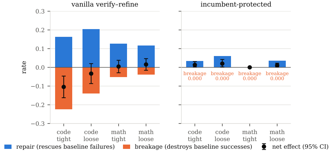
Figure 1: The decomposition, on frozen test splits. Repair (blue, above the axis) and breakage (orange, below) are of comparable size for a standard verify-refine workflow, so the net effect (black, 95% CI) sits near zero or below it — the quantity the literature reports is a difference of two large terms. Protecting the incumbent answer removes the lower term entirely (breakage 0.000 in all cells) and the same machinery becomes a small, reliable gain. Both panels share an axis.
