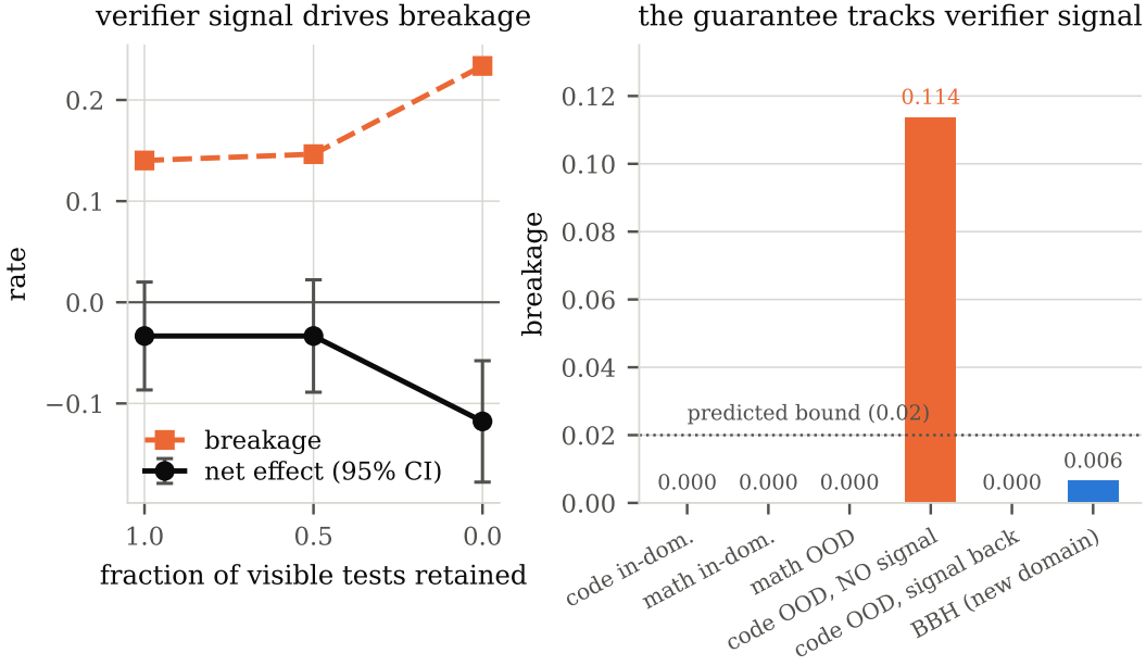
Figure 2: Left: degrading the verifier is a causal manipulation of the breakage term. As visible tests are withheld, breakage rises and the net effect falls to -0.118 [-0.178, -0.058] . Right: breakage of the incumbent-protecting construction across every condition we measured. It stays below the predicted bound wherever the verifier carries signal — including out of domain, and in a third domain whose prediction was locked before execution — and exceeds it in exactly the one condition with no signal. Restoring signal on the same tasks restores the guarantee.
