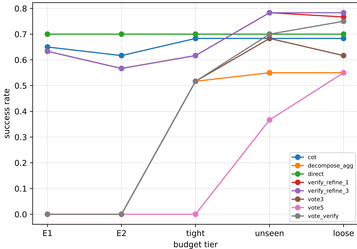
code: budget-structure envelope (dev, seed 0)
