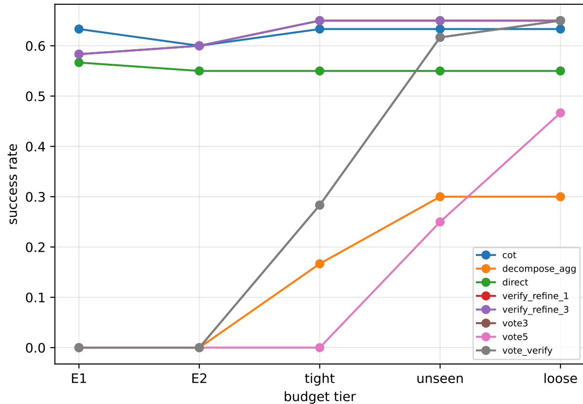
math: budget-structure envelope (dev, seed 0)
