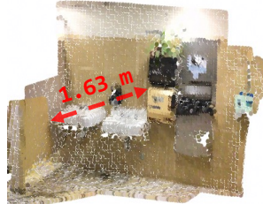
MapAnything
