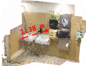
CUT3R
