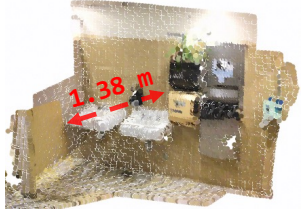
CUT3R
