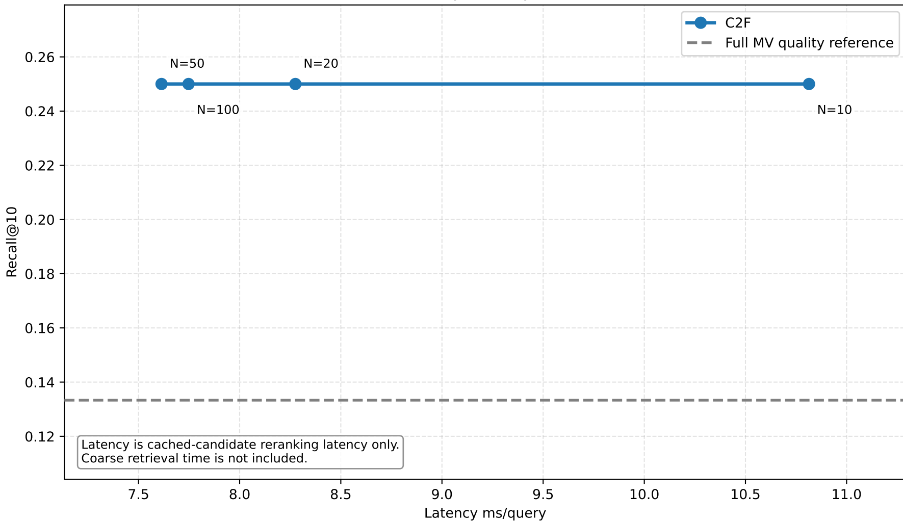
Coarse-to-Fine Quality-Latency Curve (Recall@10)
