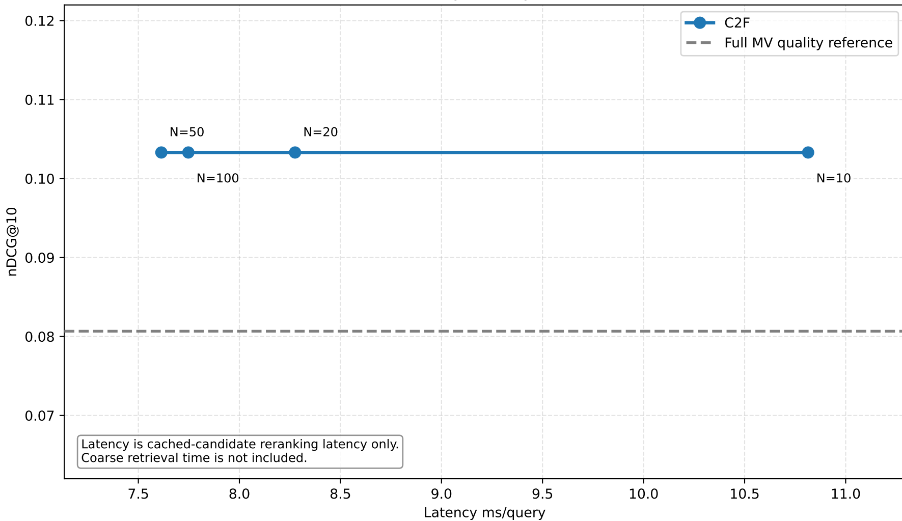
Coarse-to-Fine Quality-Latency Curve (nDCG@10)
