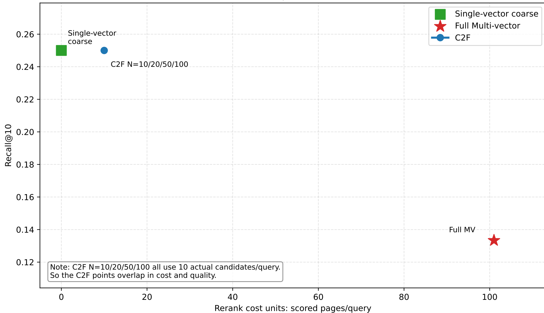
Coarse-to-Fine Quality-Cost Curve (Recall@10)
