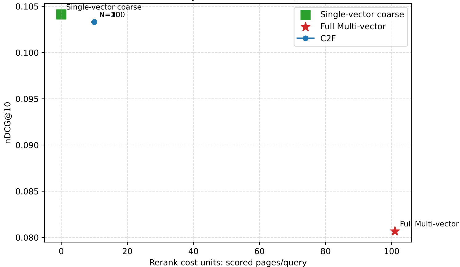
C2F Quality-Cost Curve (nDCG@10)
