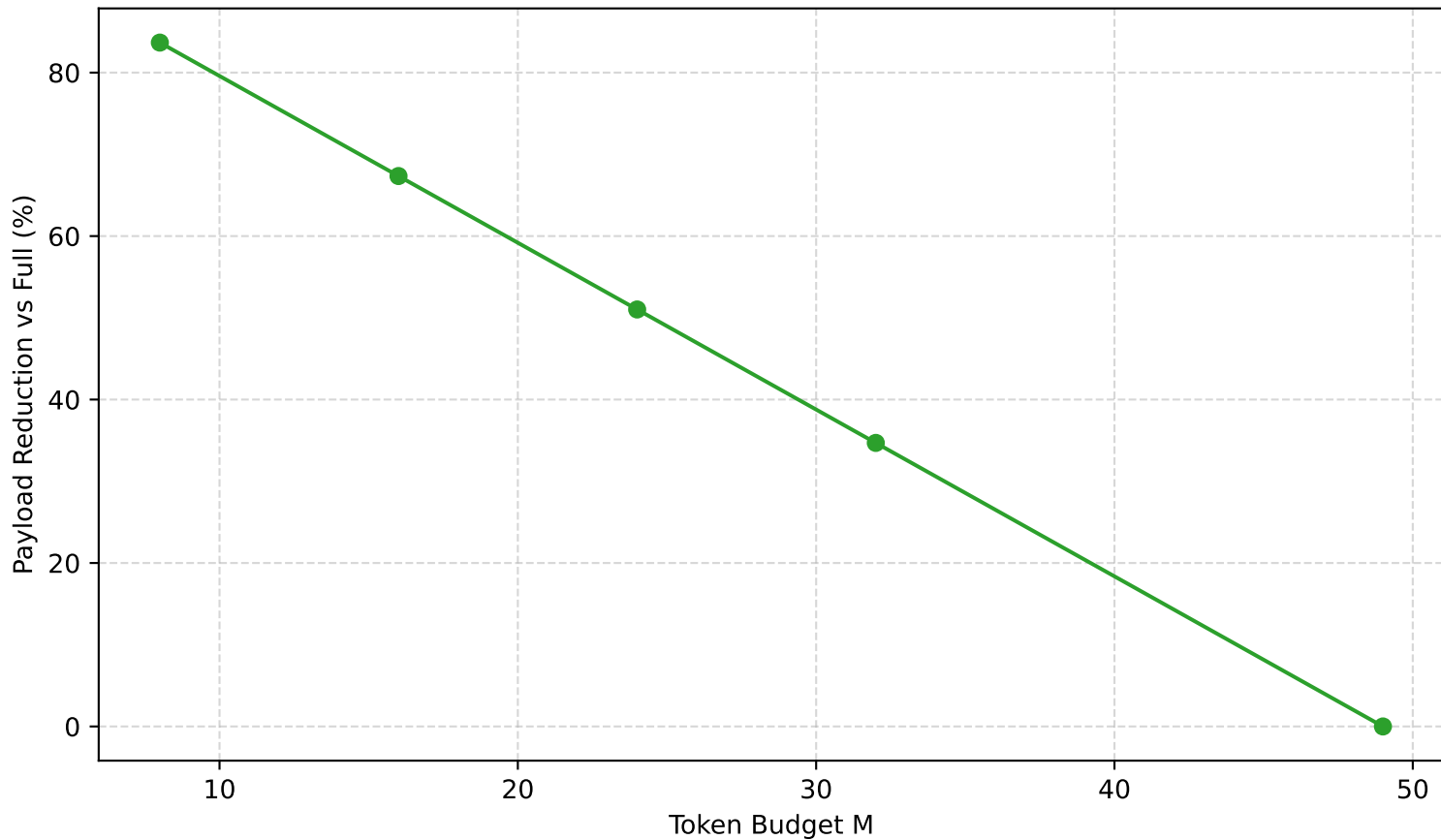
Index Size Reduction under Different Token Budgets
