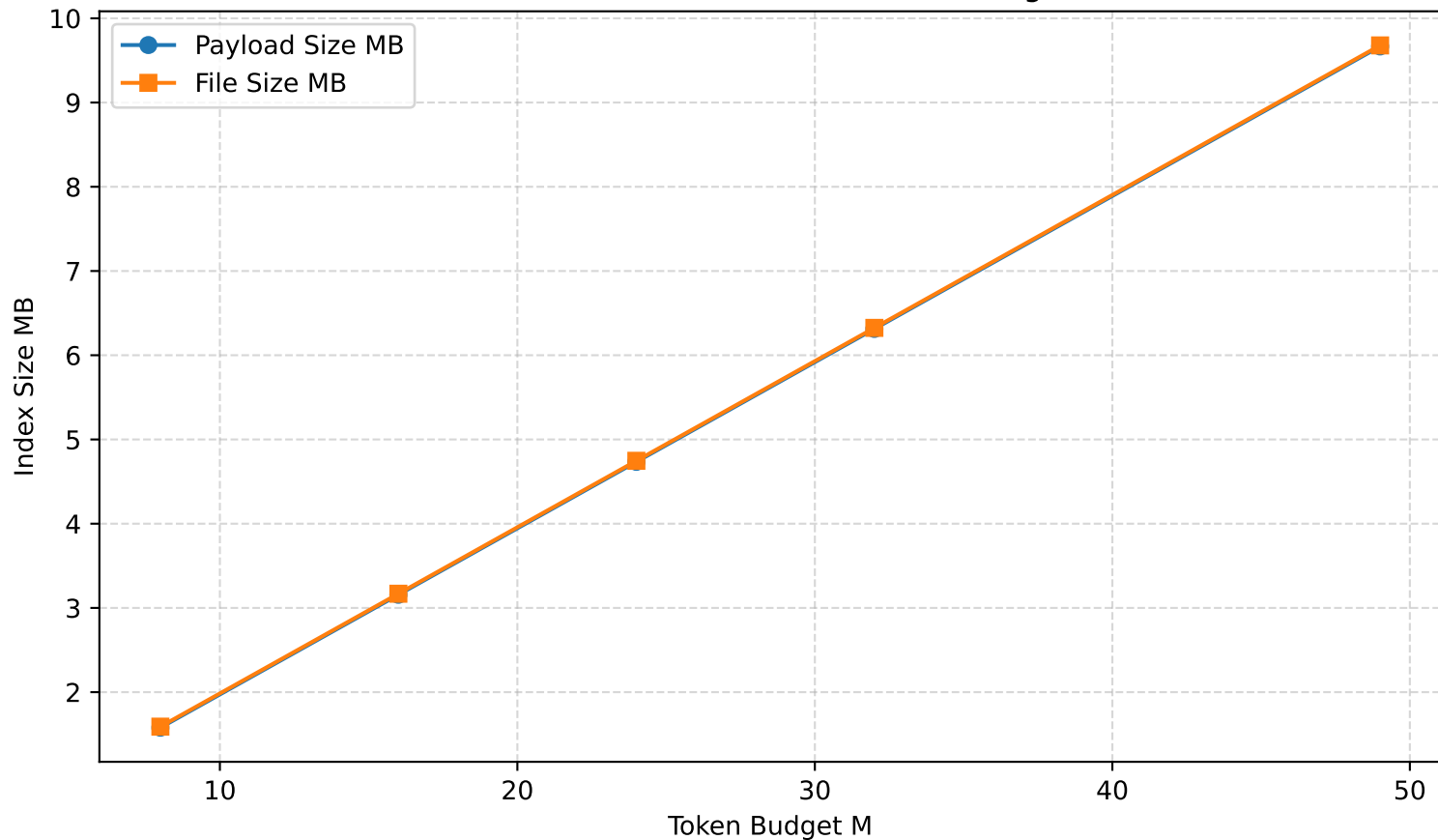
Index Size under Different Token Budgets
