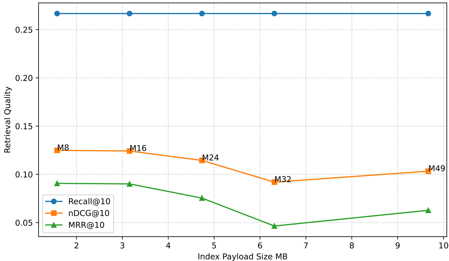
Quality vs Index Size
