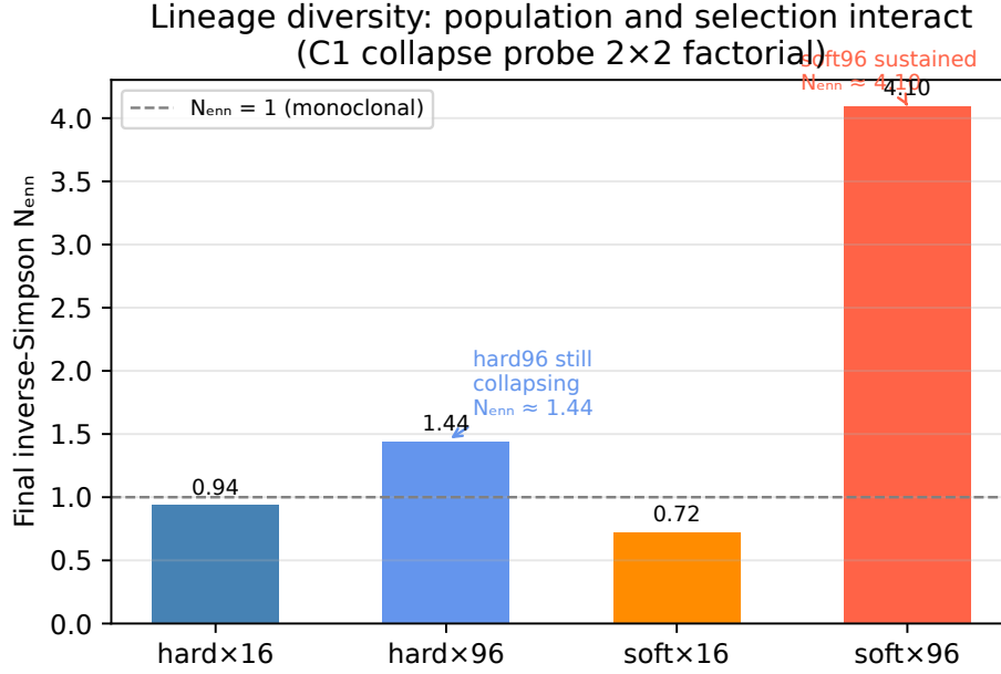
Figure 4: Final inverse-Simpson N_{\text{eff}} across the 2 \times 2 factorial (C1 collapse probe). Population size opens windows; only soft (niching) selection sustains diversity. Soft \times 96: N_{\text{eff}} \approx 4.10 (sustained); hard \times 96: N_{\text{eff}} \approx 1.44 (still collapsing). Source: rtc_g1f_c1_collapse_probe_verdict.json .
