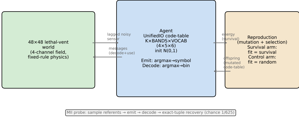
Substrate schematic: lethal-vent world, tied code-table agent, and evolution loop
