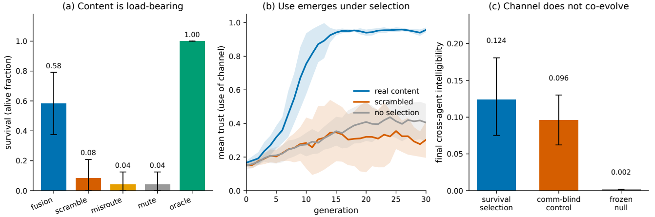
Figure 1: Results inside the constructed world; all values from committed verdict artifacts, bars are bootstrap 95% CIs. (a) Lethal signaling (24 seeds): fusion (real decoded content, 0.58) survives far above scramble (random, 0.08), misroute (correct content, broken content-to-location binding, 0.04) and mute (0.04); oracle (fenced) = 1.00. fusion beats each control by an exact paired McNemar test ( p < 5e-4 ); the run’s own absolute-majority gate is inconclusive, so this is a relative result, and misroute isolates that content-to-location binding (not signal presence) carries survival. (b) A heritable “trust” gene (8 seeds) rises to \approx 0.96 under real content vs. \sim 0.3 – 0.4 under scrambled / no selection: use of a separately-trained channel is selected for (adoption, not de-novo emergence). (c) Co-evolving the channel from random weights (6 seeds): the apparent intelligibility rise (0.124) does not separate from a communication-blind control (0.096; survival–control CI [-0.05, 0.11] includes 0), both far above the frozen null (0.002)—clonal descent-convergence, not selection for communication.
