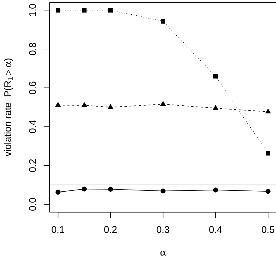
Violation rate vs nominal delta = 0.1
