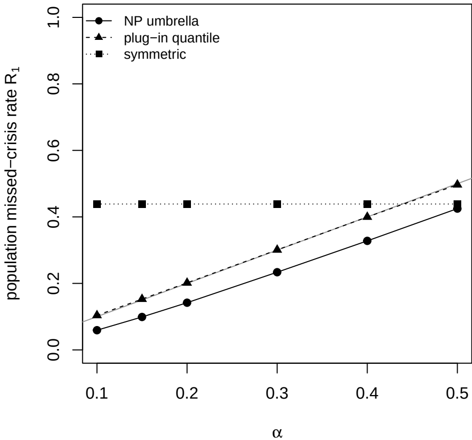
Realized type II error (n = 4000)
