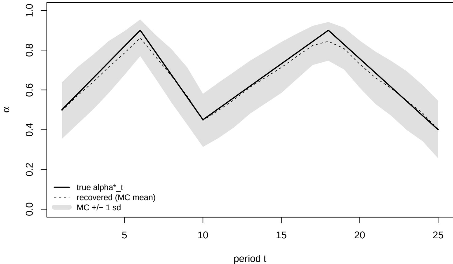
True vs recovered risk tolerance
