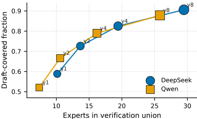
(c) Longer drafts amplify expert demand
