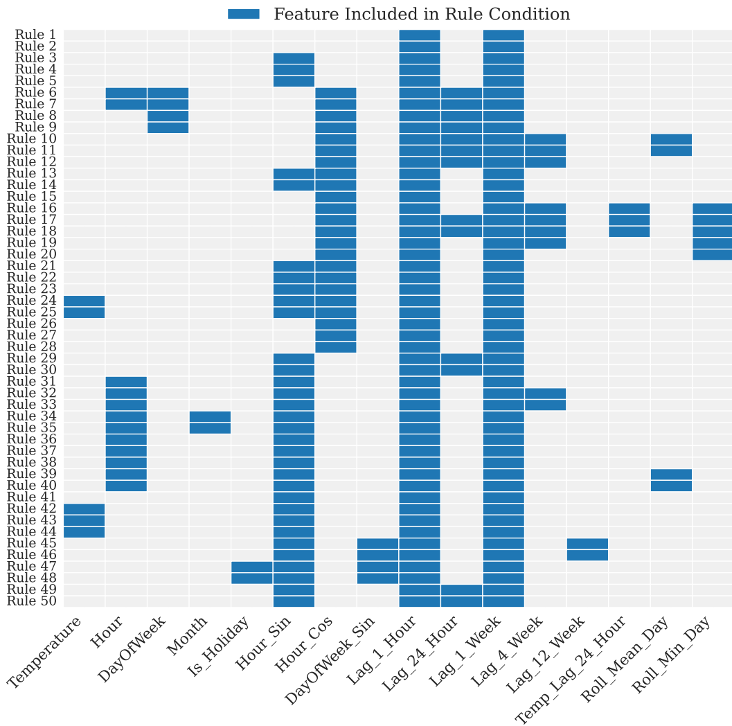
Extracted Top Rules
