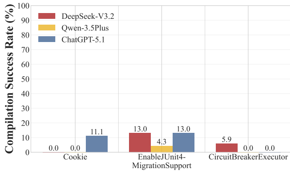
Figure 3: Effectiveness of C++-to-Java Translation using LLMs with Method-by-method Strategy w.r.t Project and Modules
