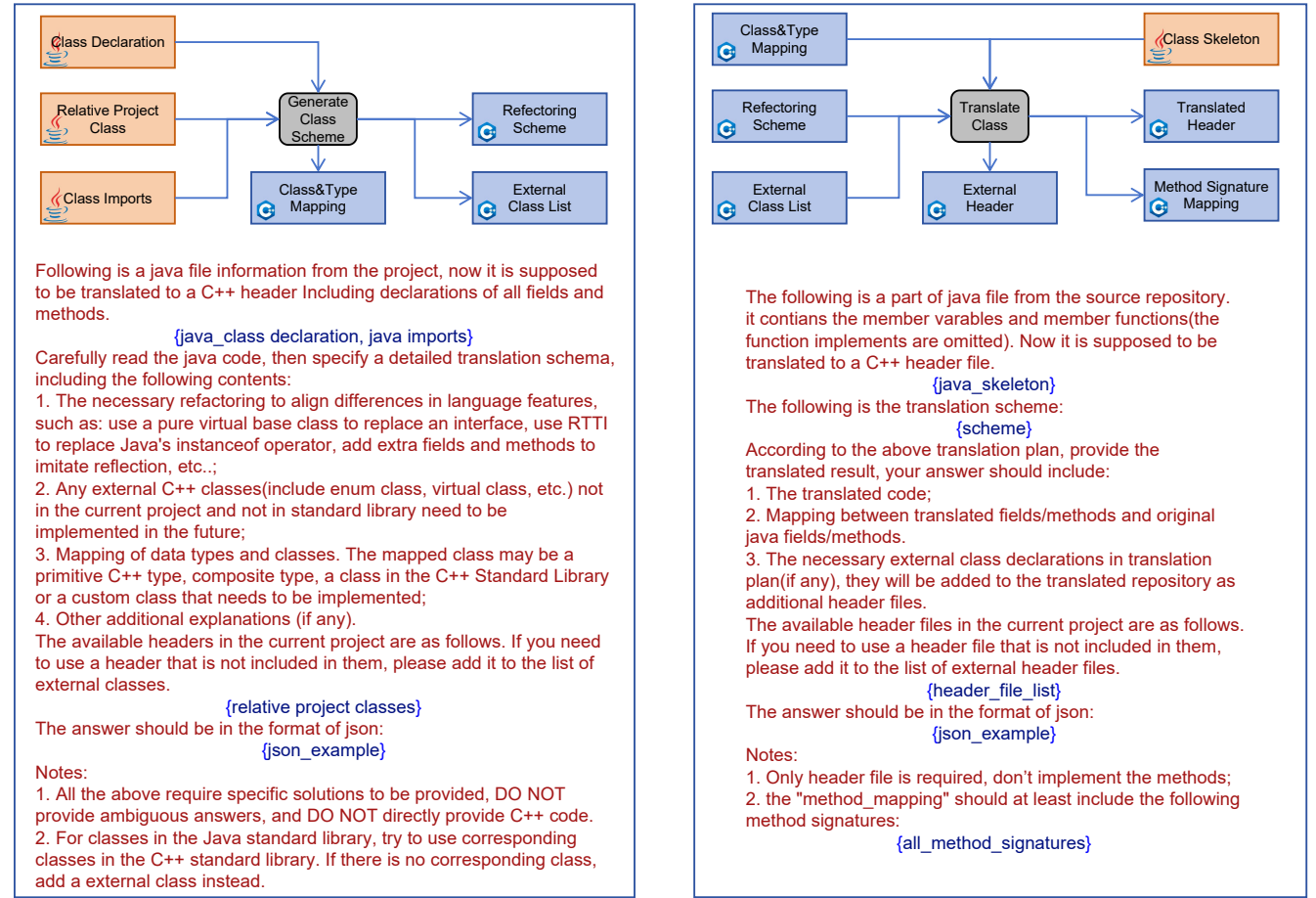
Figure 3: Header-level translation scheme and data flow. The LLM analyzes the Java class structure, generates a translation scheme specifying type mappings and structural changes, then produces the corresponding C++ header file.
