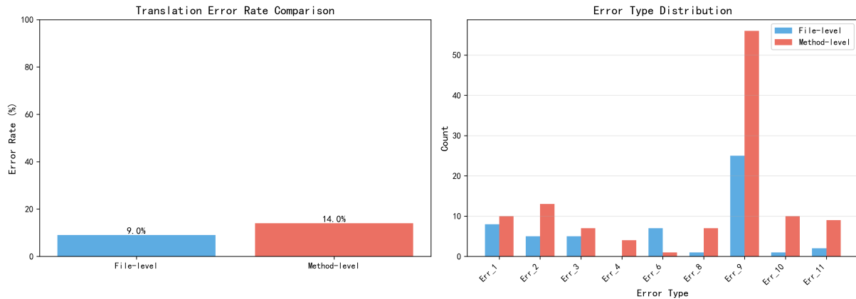
Figure 1: Error type distribution in File-level vs Method-level translation
