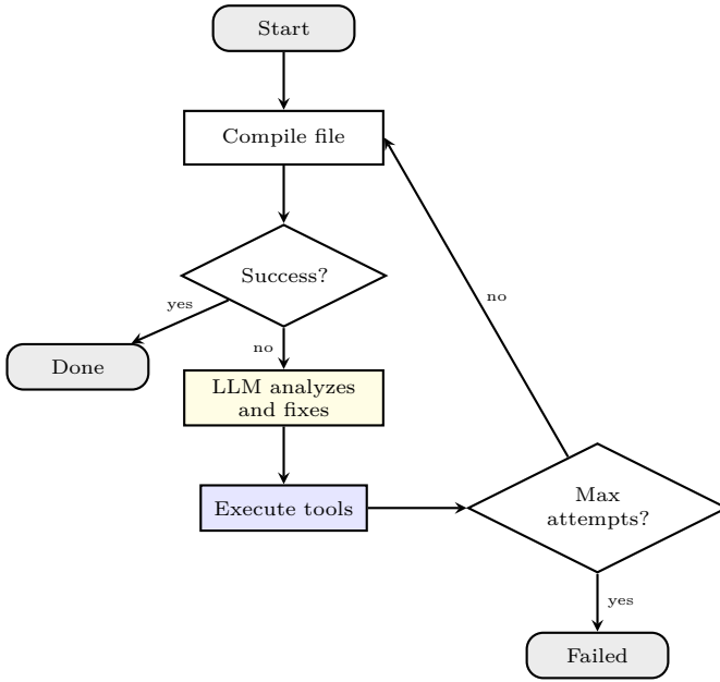
Figure 5: The compilation agent’s iterative repair process.
