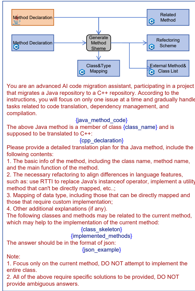
Figure 4: Method-level translation scheme and data flow. The bottom-up translation order ensures that callee methods are translated before callers, enabling context propagation where already-translated code serves as reference.
