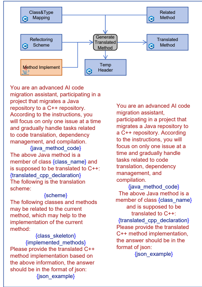
Figure 4: Method-level translation scheme and data flow. The bottom-up translation order ensures that callee methods are translated before callers, enabling context propagation where already-translated code serves as reference.
