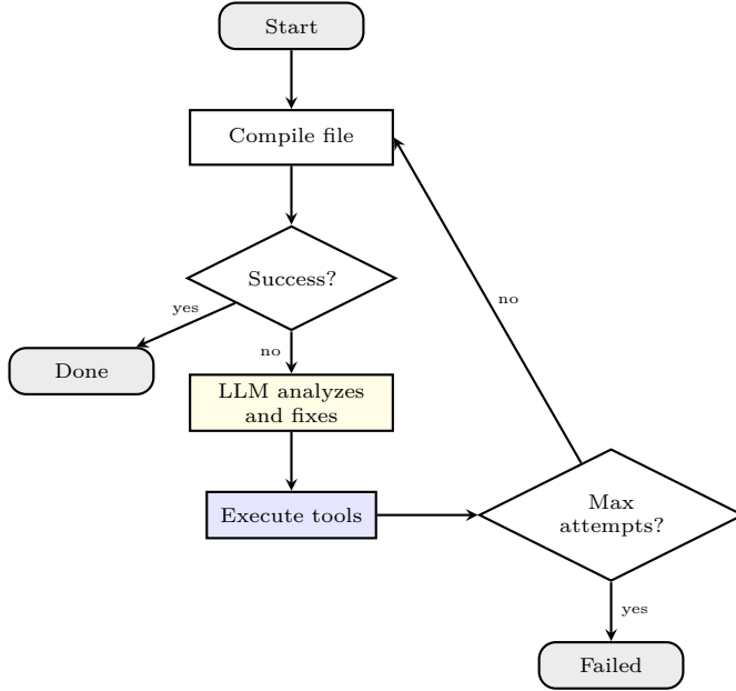
Figure 8: The compilation agent’s iterative repair process.
