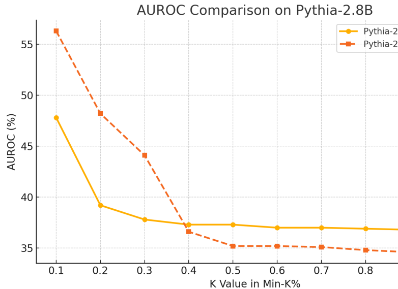
Figure 1: AUROC performance under Hyperparameter K
