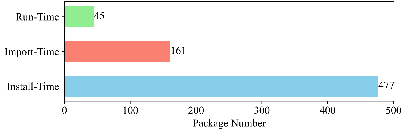
PyPI Triggering Scenarios
