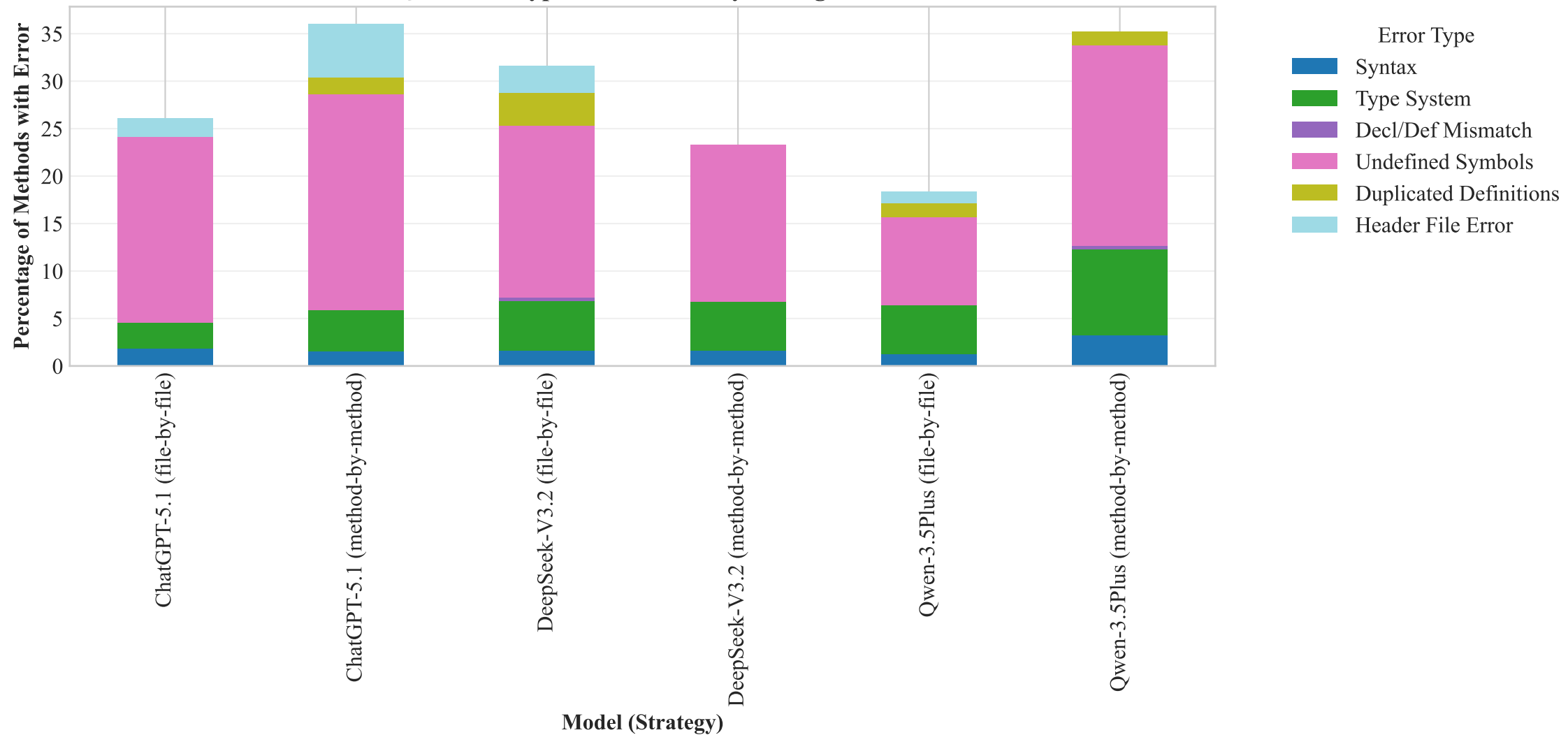
RQ2: Error Type Distribution by Configuration
