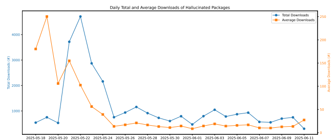
Figure 4: Daily total and average downloads of hallucinated packages.
