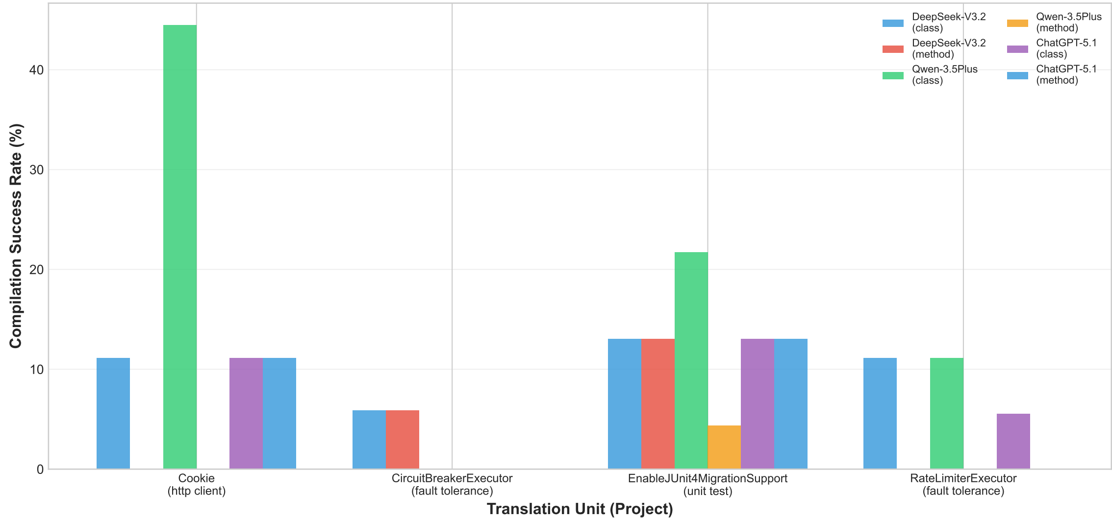
RQ1: Success Rate Across Different Projects
