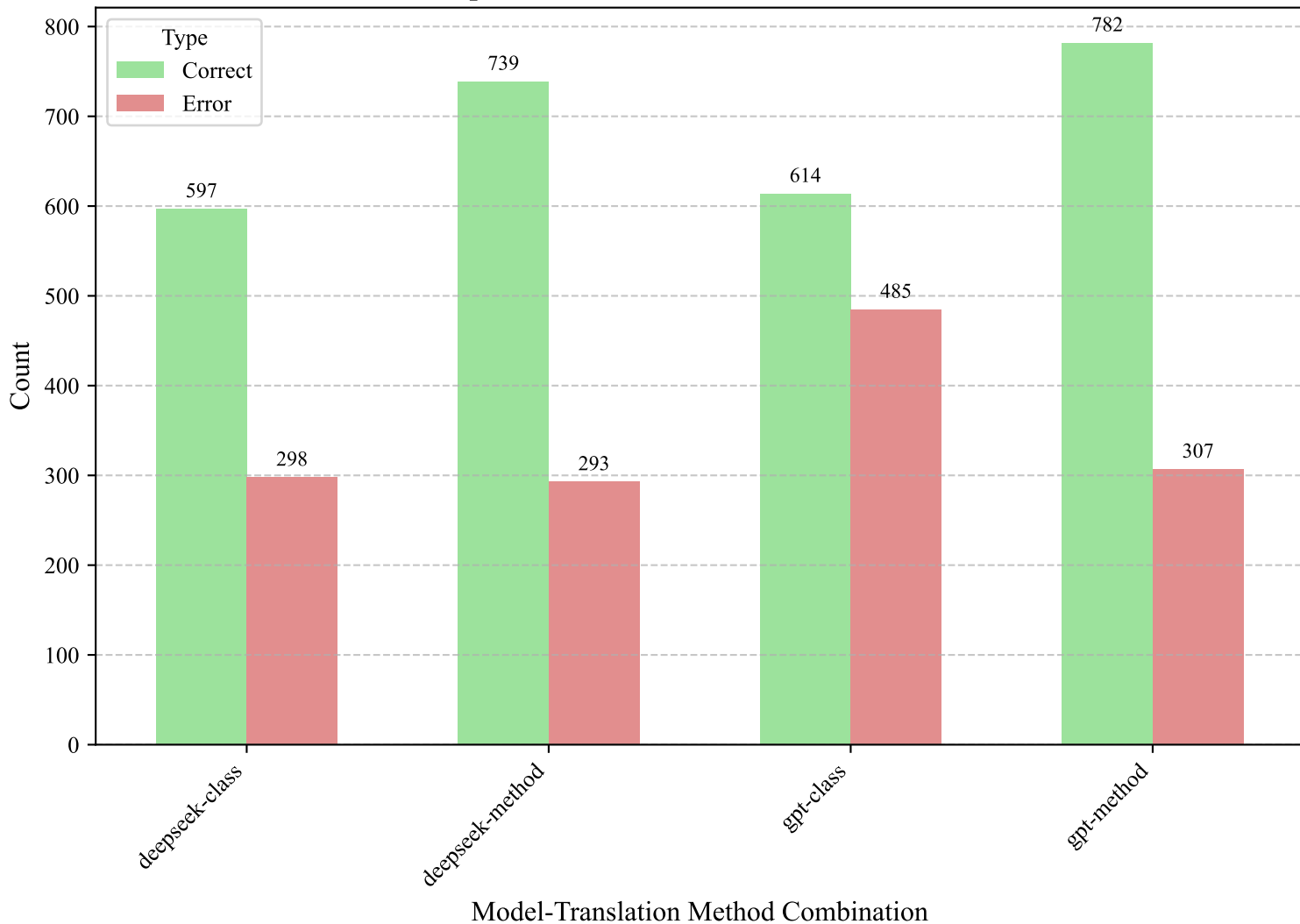
Correctness Comparison of Model-Translation Method Combinations
