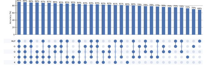
Figure 1: Accuracy of lineage detection with different combinations of transformer block components (RQ2).
