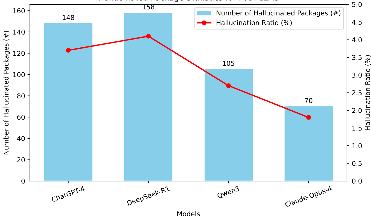
Hallucinated Package Statistics for Four LLMs
