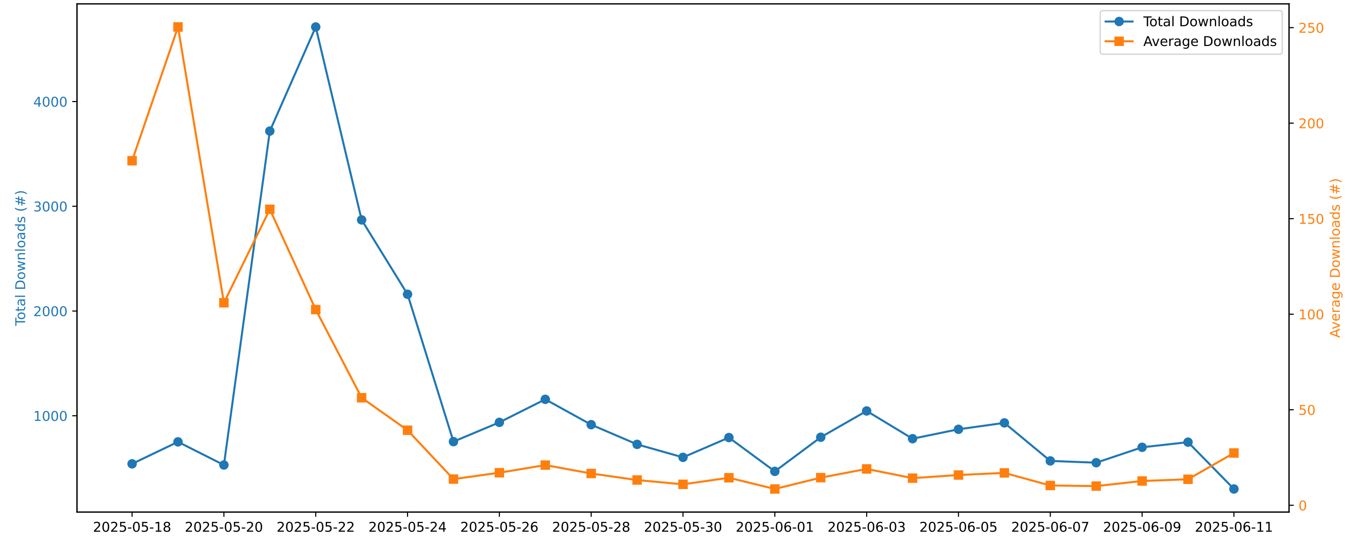
Daily Total and Average Downloads of Hallucinated Packages
