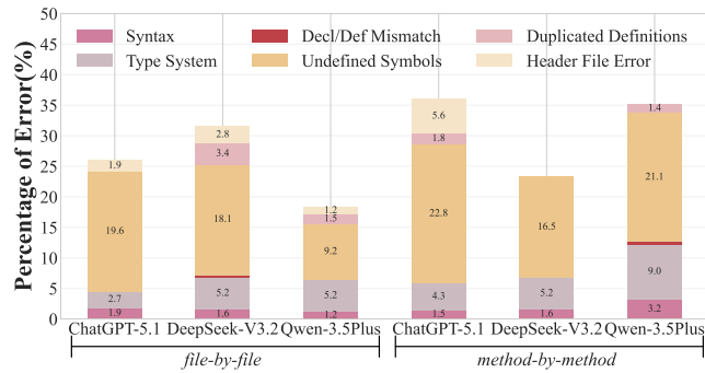
Figure 5: Stacked Error Distribution at Method Level
