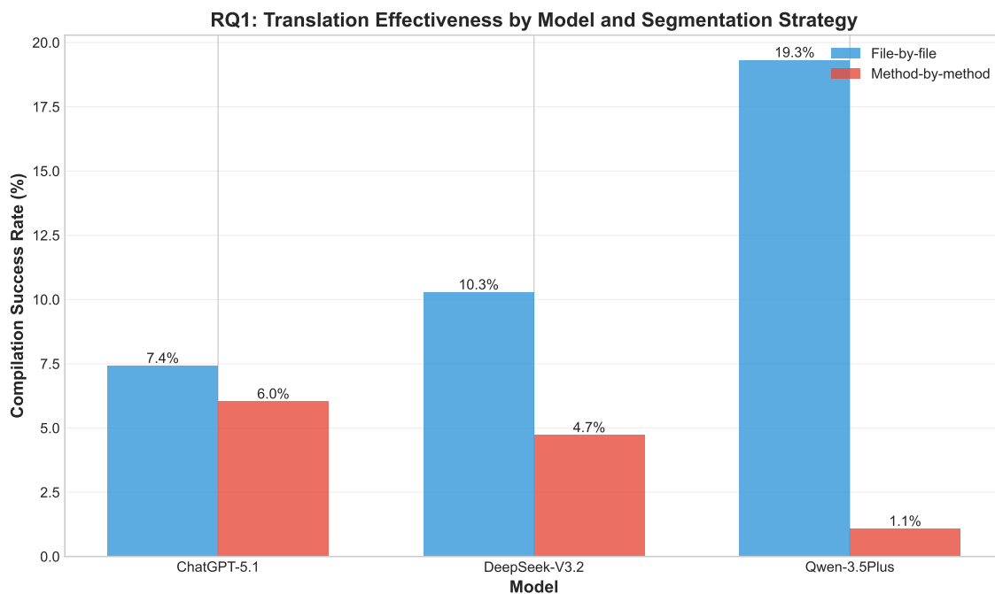
Figure 1: Overall compilation success rates by model and segmentation strategy. File-by-file translation generally outperforms method-by-method across all models.
