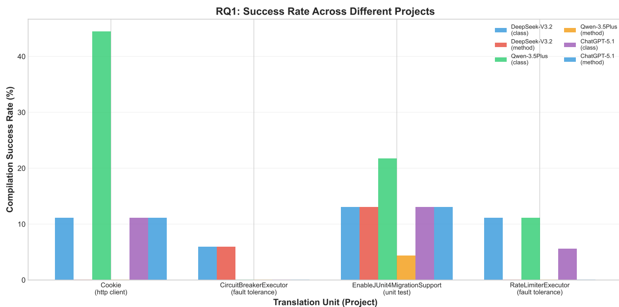
Figure 2: Compilation success rates across different projects. Performance varies significantly by translation unit, reflecting differences in code complexity and domain-specific patterns.
