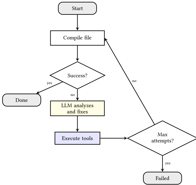
Figure 8: The compilation agent’s iterative repair process.
