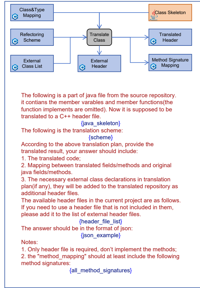
Figure 6: Header-level translation scheme and data flow. The LLM analyzes the Java class structure, generates a translation scheme specifying type mappings and structural changes, then produces the corresponding C++ header file.
