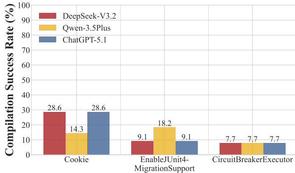
Figure 2: Effectiveness of C++-to-Java Translation using LLMs with File-by-file Strategy w.r.t Project and Modules
