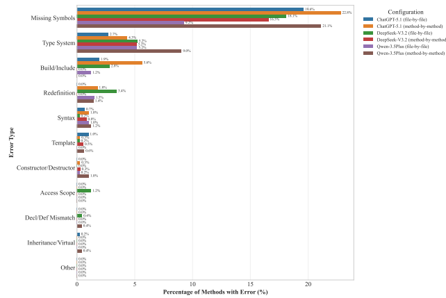
Figure 4: Error Type Distribution at Method Level Across Models and Strategies
