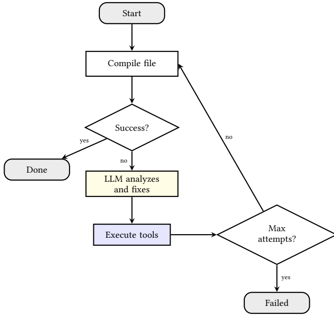
Figure 11: The compilation agent’s iterative repair process.
