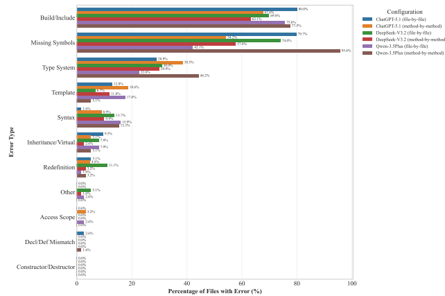
Figure 5: Error Type Distribution at Class Level Across Models and Strategies
