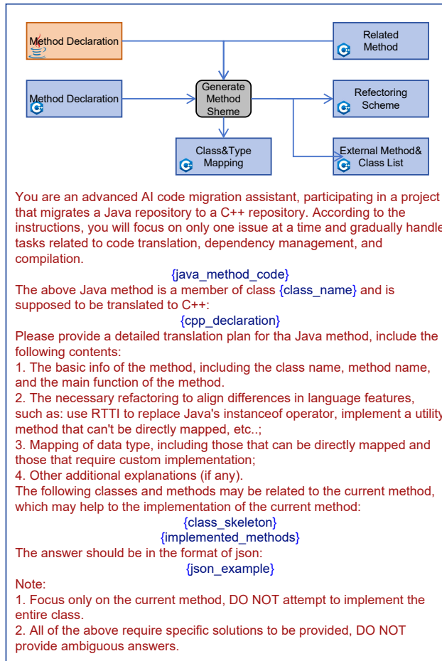
Figure 10: Method-level translation scheme and data flow. The bottom-up translation order ensures that callee methods are translated before callers, enabling context propagation where already-translated code serves as reference.
