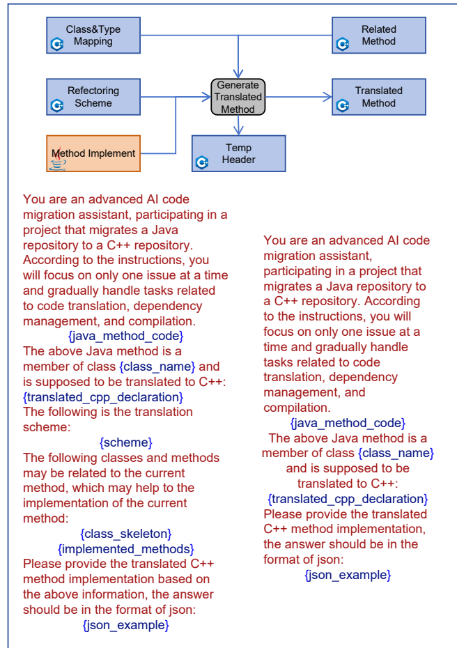
Figure 10: Method-level translation scheme and data flow. The bottom-up translation order ensures that callee methods are translated before callers, enabling context propagation where already-translated code serves as reference.
