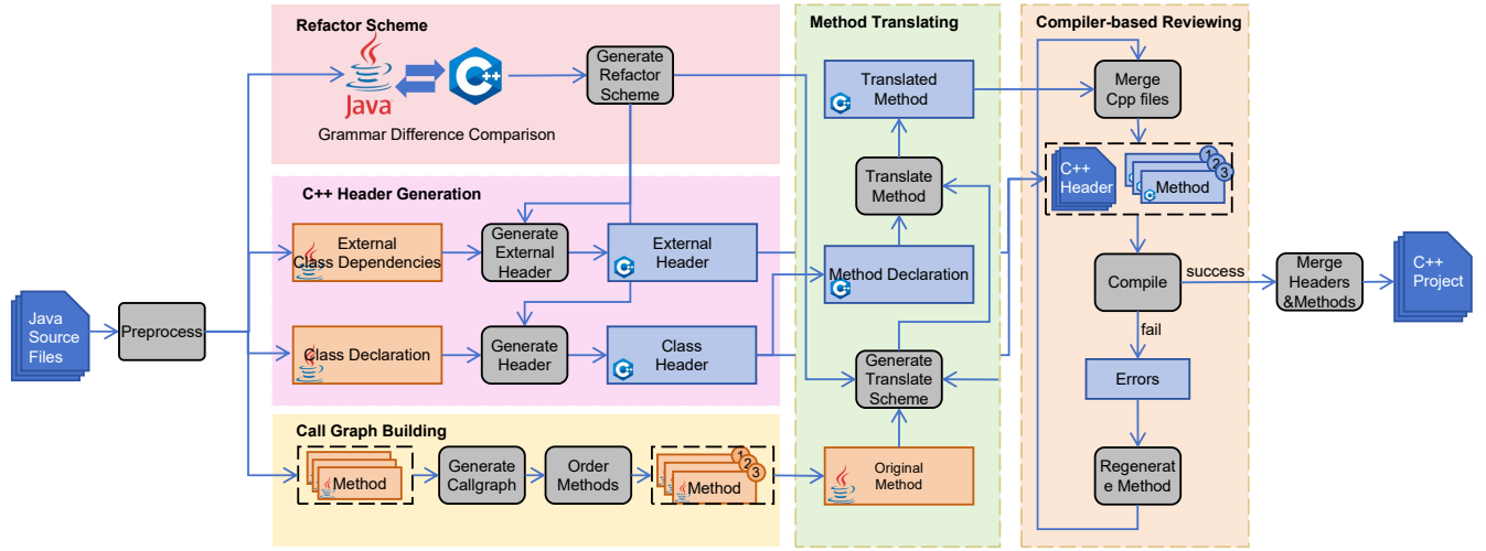
Figure 8: Overall architecture of TOOL showing the three-phase translation process.
