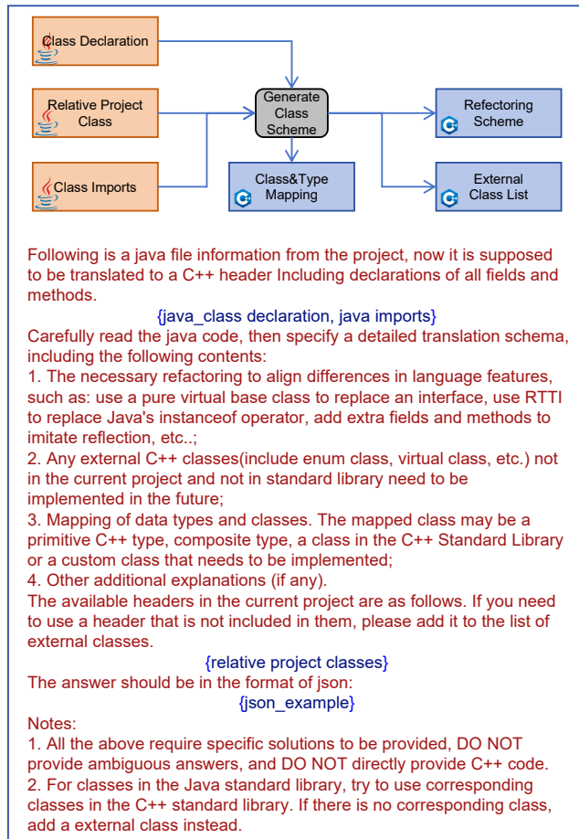
Figure 9: Header-level translation scheme and data flow. The LLM analyzes the Java class structure, generates a translation scheme specifying type mappings and structural changes, then produces the corresponding C++ header file.
