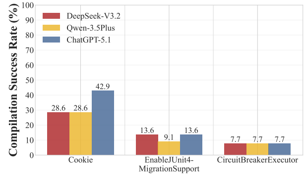
Figure 3: Effectiveness of C++-to-Java Translation using LLMs with Method-by-method Strategy w.r.t Project and Modules
