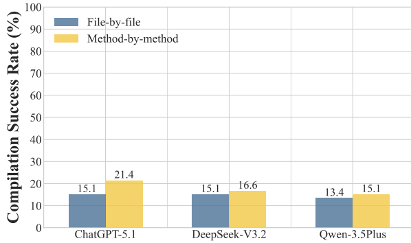
Figure 1: Effectiveness of C++-to-Java Translation using LLMs under Two Translation Strategies
