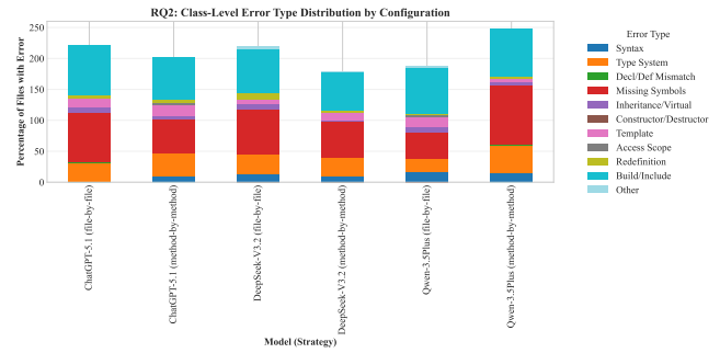
Figure 7: Stacked Error Distribution at Class Level
