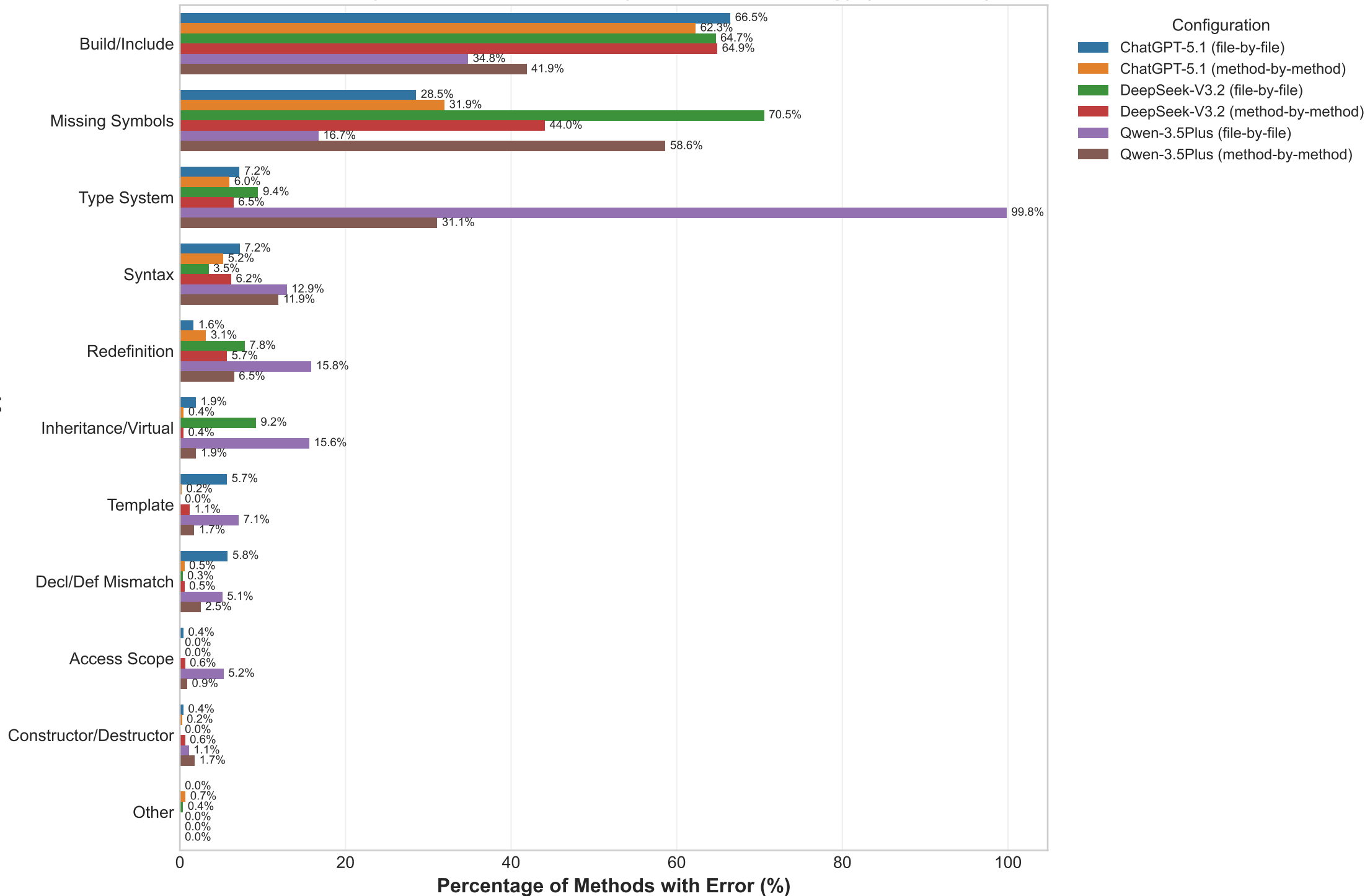
RQ2: Error Type Occurrence Rate by Model and Strategy (Horizontal)
