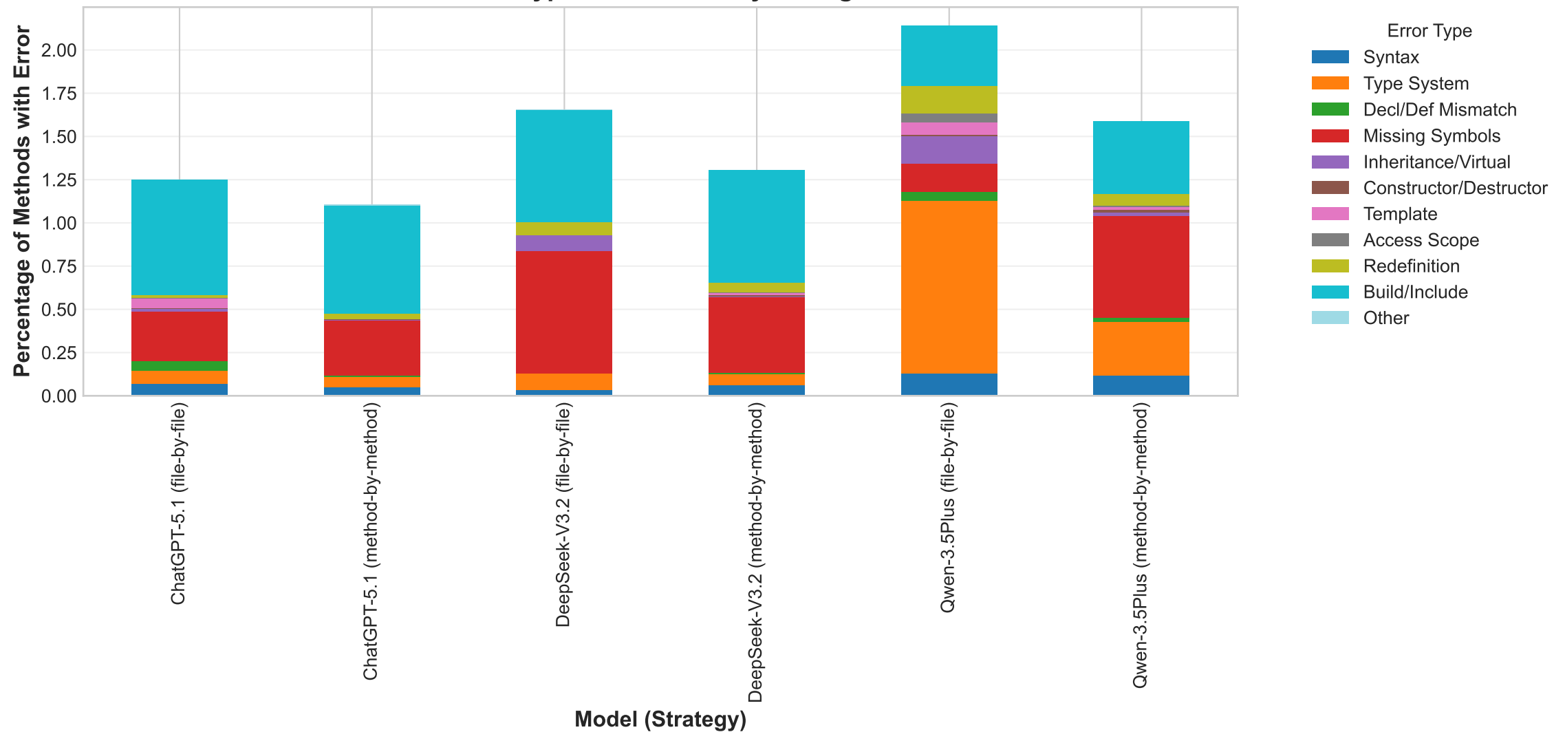
RQ2: Error Type Distribution by Configuration
