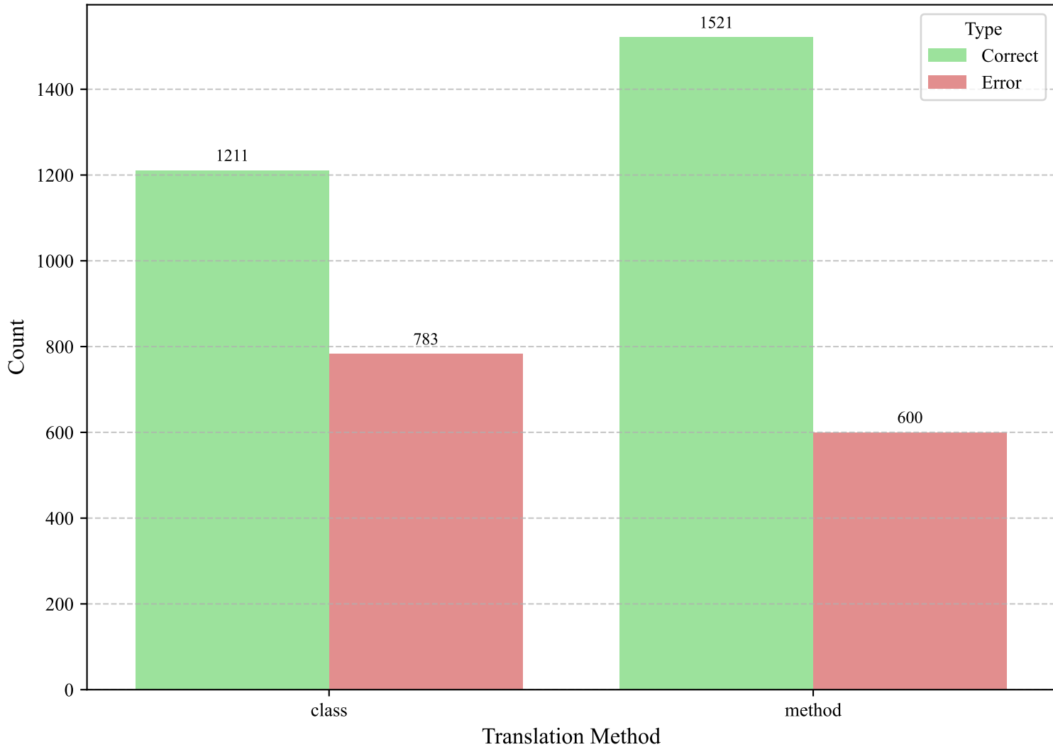
Class vs. Method Translation Method Correctness Comparison Across All Models
