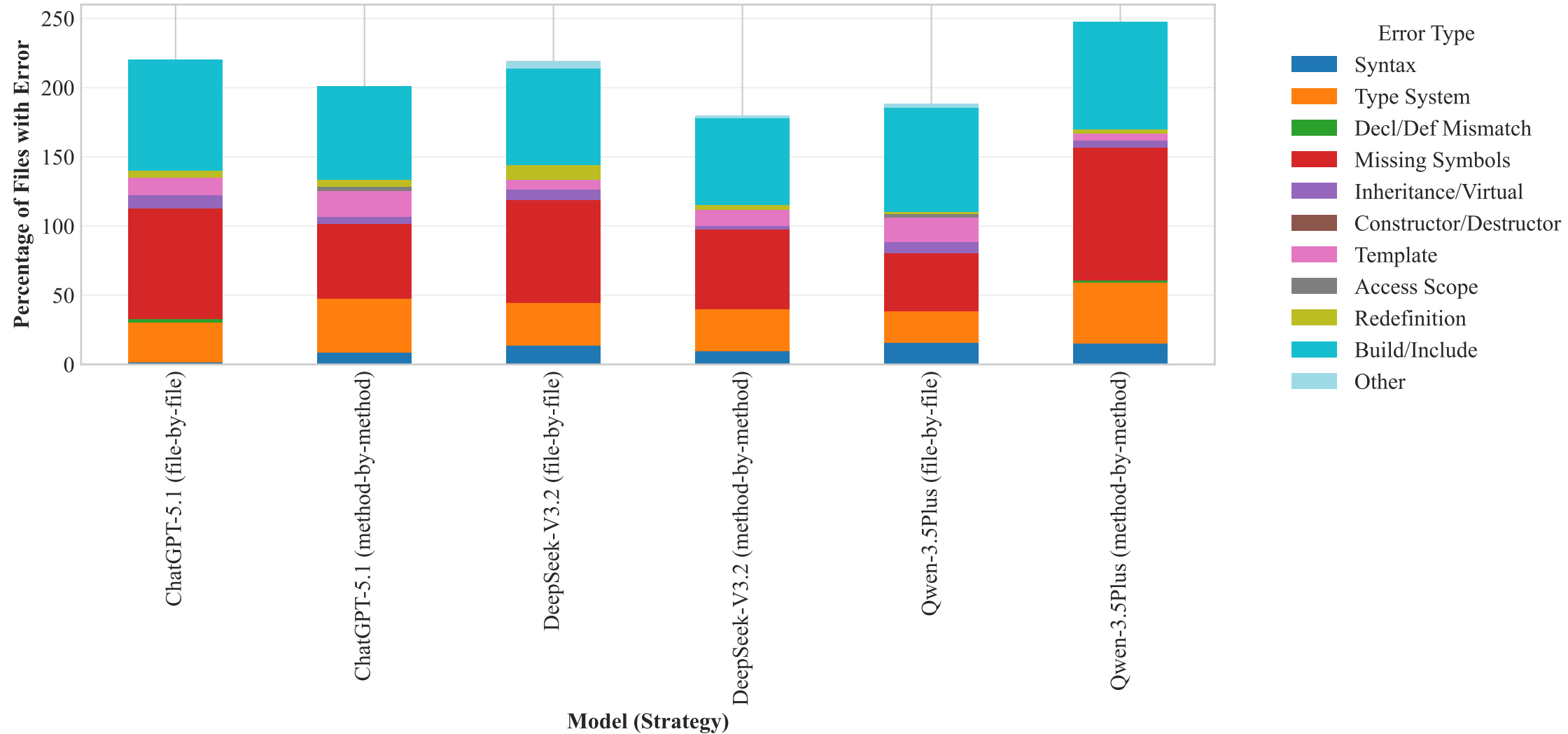
RQ2: Class-Level Error Type Distribution by Configuration
