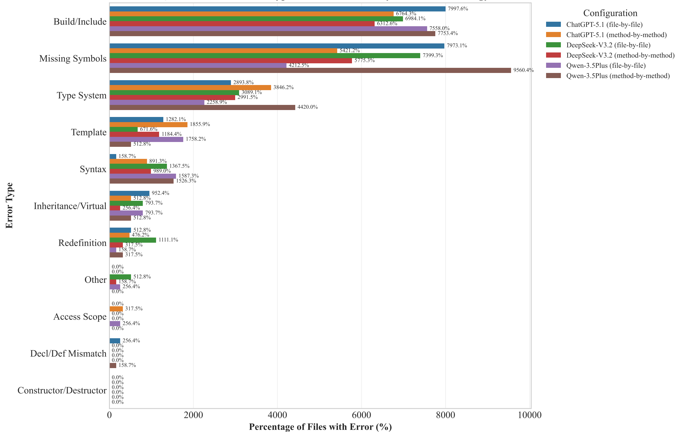
RQ2: Class-Level Error Type Occurrence Rate by Model and Strategy
