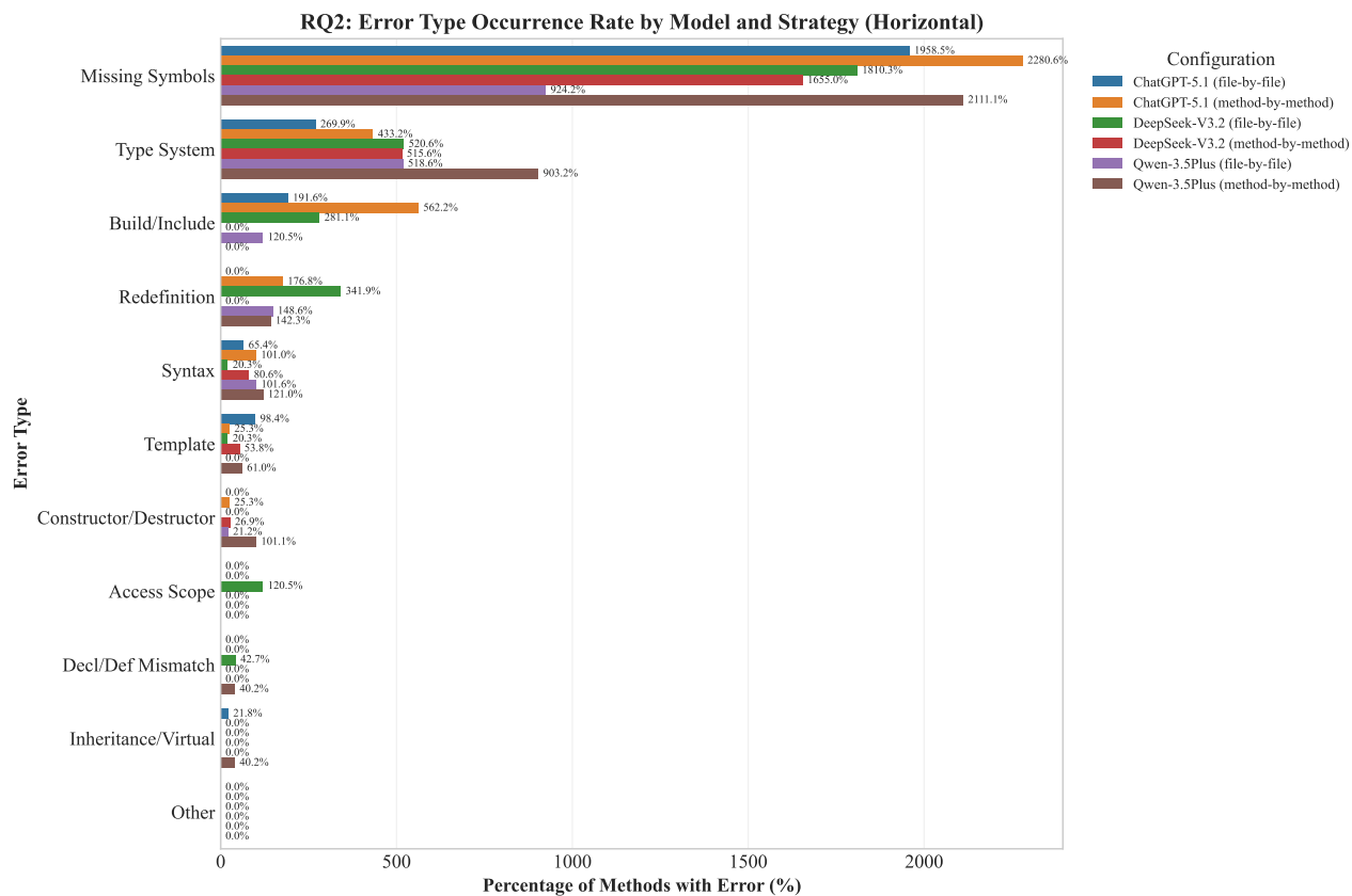
Figure 5: Error type occurrence rate by model and translation strategy (Method-Level).
