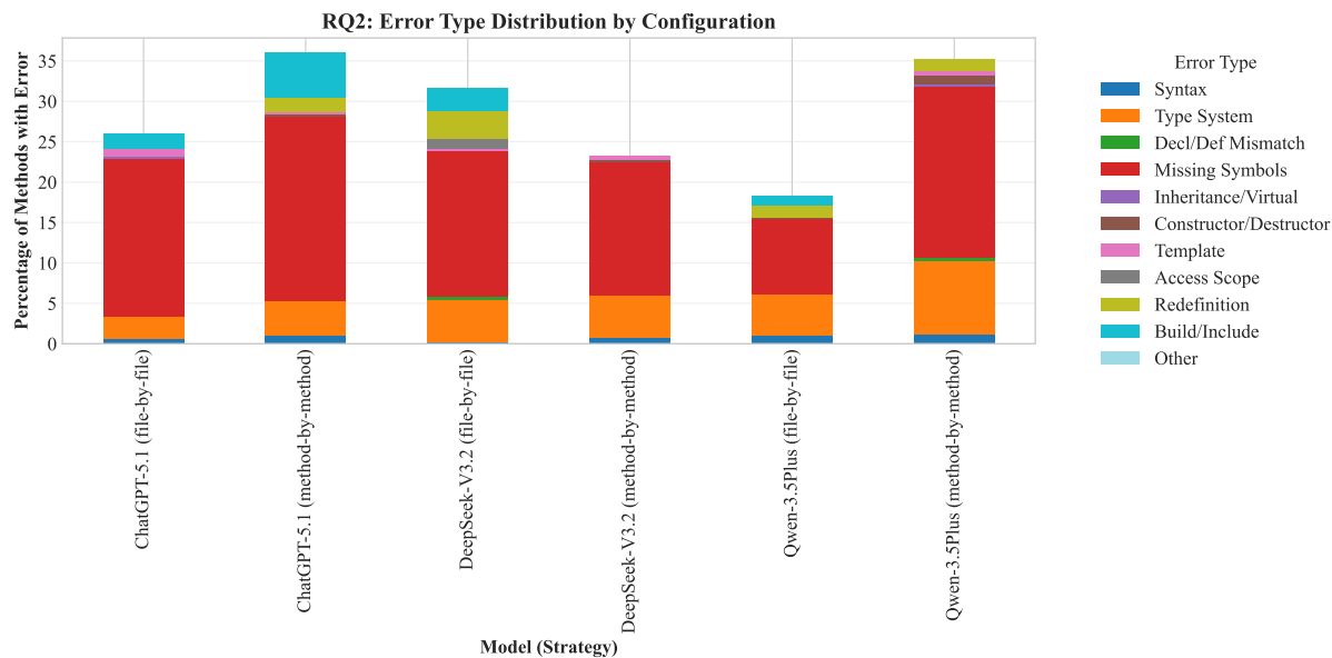
Figure 6: Stacked error distribution by configuration(method-level). Each bar shows the percentage of methods containing each error type.
