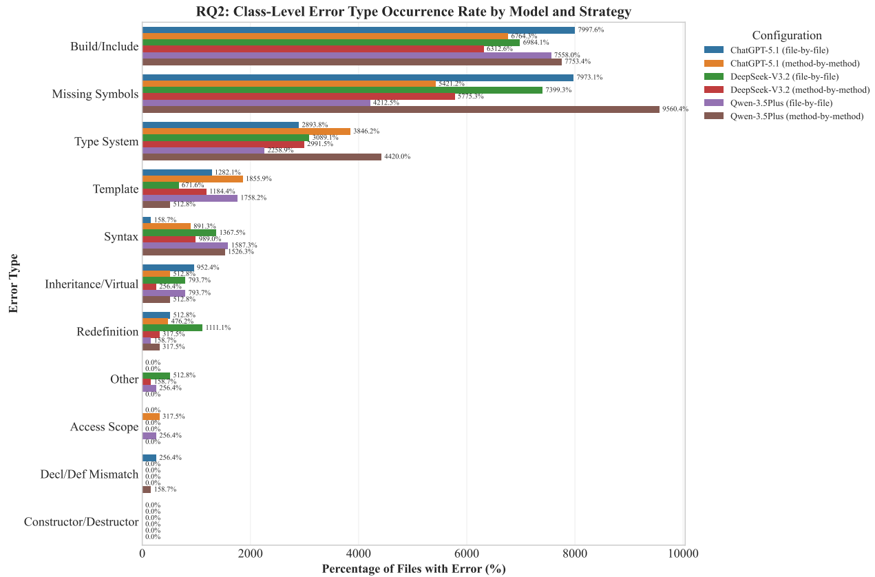
Figure 4: Error type occurrence rate by model and translation strategy (Class-Level).
