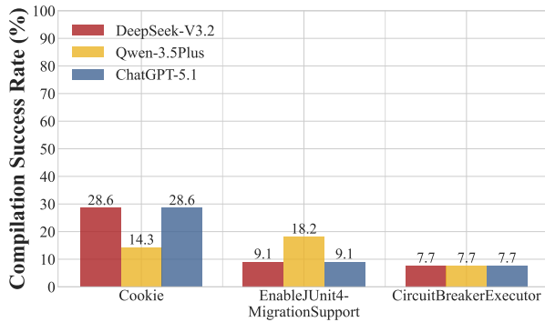
Figure 2: Effectiveness of C++-to-Java Translation using LLMs with File-by-file Strategy w.r.t Project and Modules
