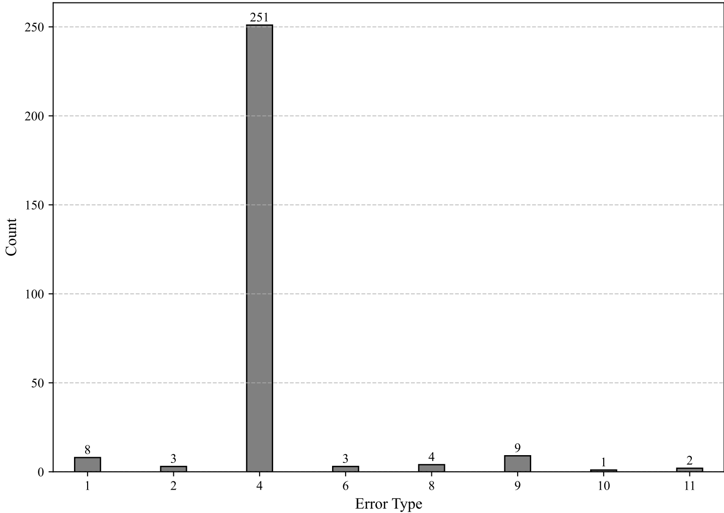
deepseek-class_Method_Error_Analysis Error_Type_Distribution - Bar Chart
