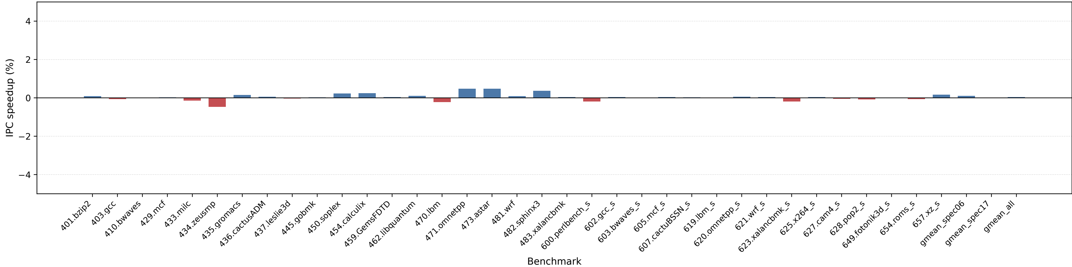
Permit PGC + CP-PB IPC speedup over Permit PGC
